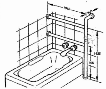
Double bar wall-mounted bath rail HT6
